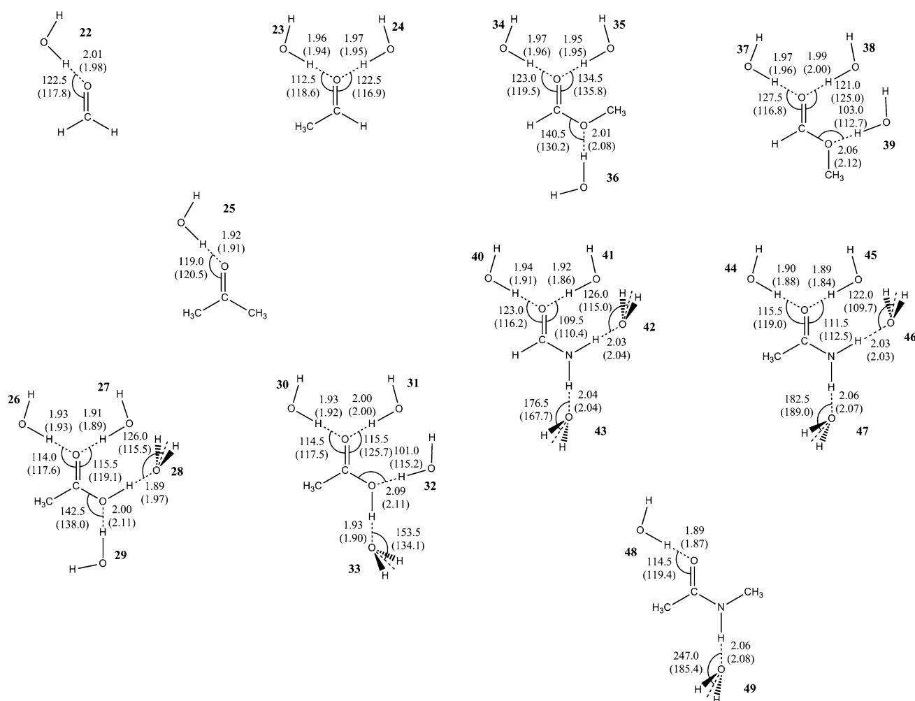
Fig. 2 Bimolecular complexes depicting the interactions between water and a series of carbonyl-containing compounds. Optimized hydrogen bond distances and angles from the X-Pol potential,
