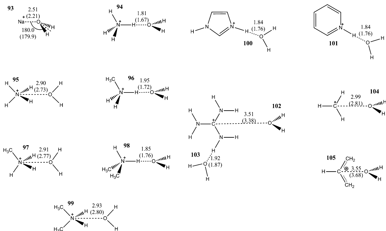
Fig. 5 Bimolecular complexes depicting the interactions between water and cationic species. Optimized hydrogen bond distances and angles from the X-Pol potential, XP@B3LYP/6-31G(d), are given
