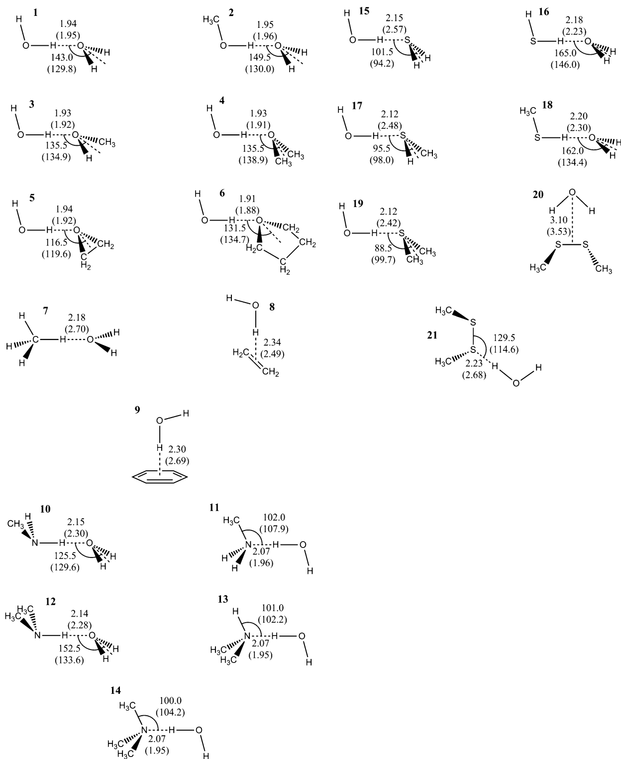
Fig. 1 Schematic illustration of the bimolecular complexes between water and small molecules. Optimized hydrogen bond distances and angles from the X-Pol potential, XP@B3LYP/6-31G(d), are first
