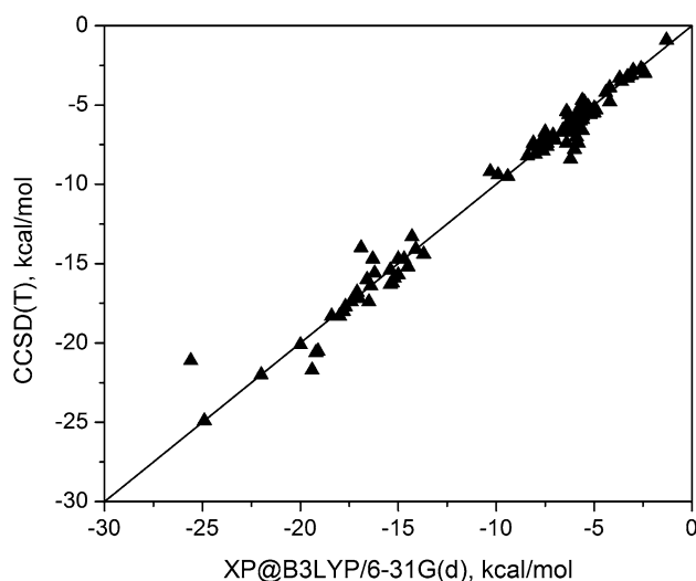
Fig. 6 Comparison of the computed hydrogen bond interaction energies obtained using the XP@B3LYP/6-31G(d) and CCSD(T)/aug-cc-pVDZ//B3LYP/aug-cc-pVDZ methods. The geometries used in the X-Pol calculations were obtained at the same level of theory, whereas those used in the coupled cluster energy evaluations were optimized with B3LYP/aug-cc-pVDZ
