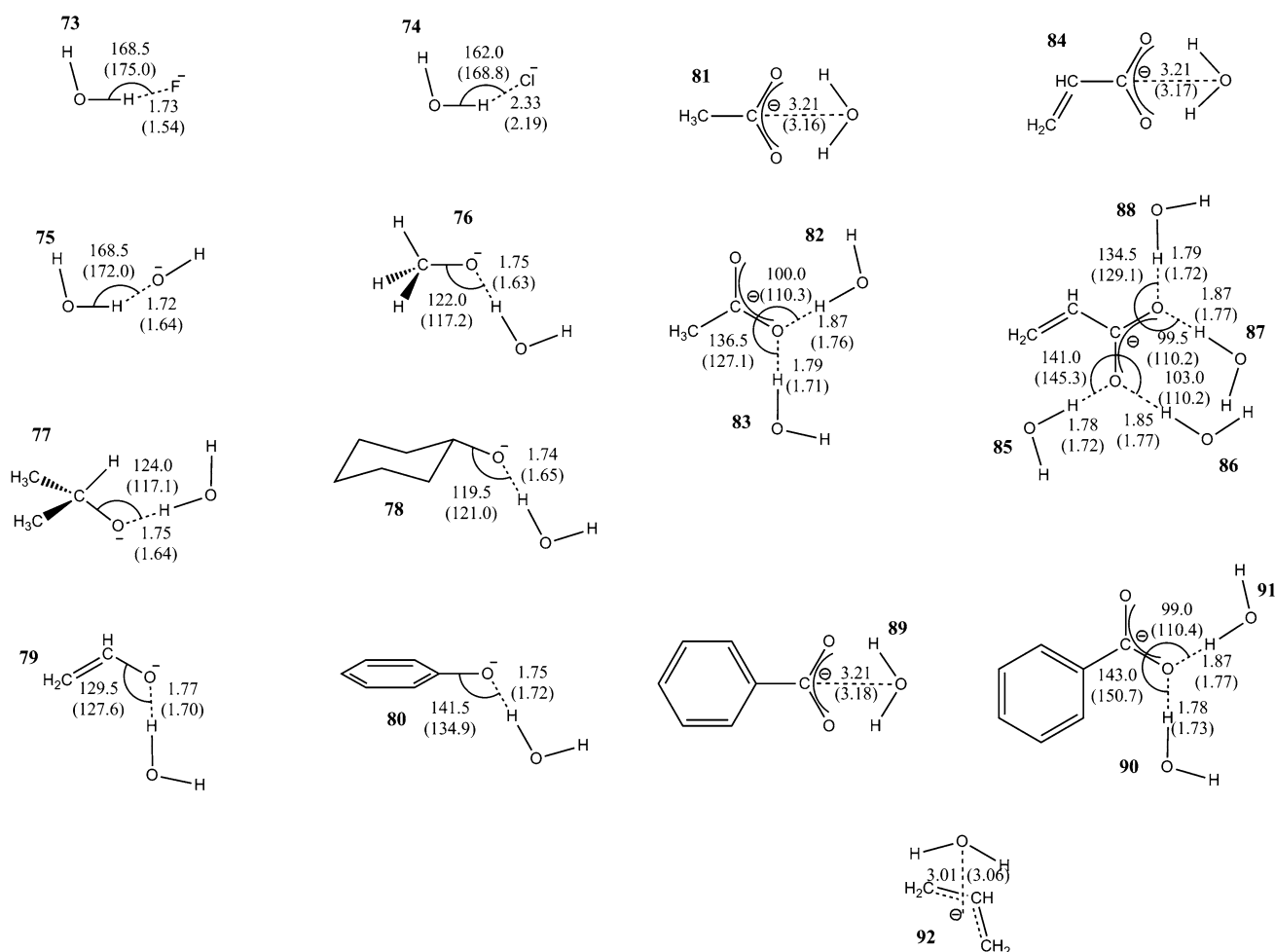
Fig. 4 Bimolecular complexes depicting the interactions between water and anionic species. Optimized hydrogen bond distances and angles from the X-Pol potential, XP@B3LYP/6-31G(d), are given
